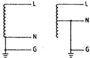
Single Phase L-N, 2 W + G
